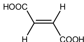
acide fumarique
